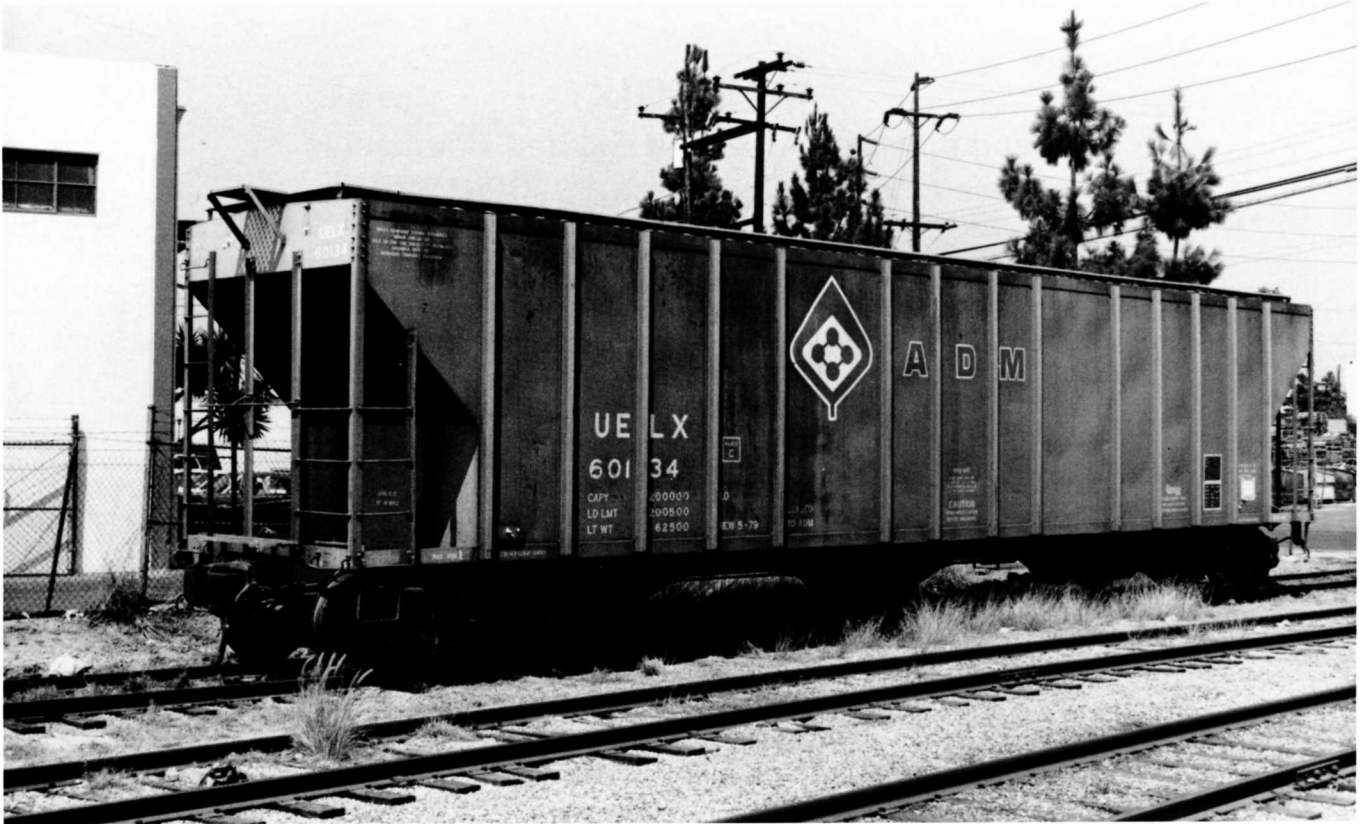
(Above) UELX 60134 was built in May 1979 by Evans. This is a 4780 cubic foot design covered hopper. Note the "Leased to ADM" on the bottom of the panel under the logo. UELX cars were originally not included on the ADM roster.
