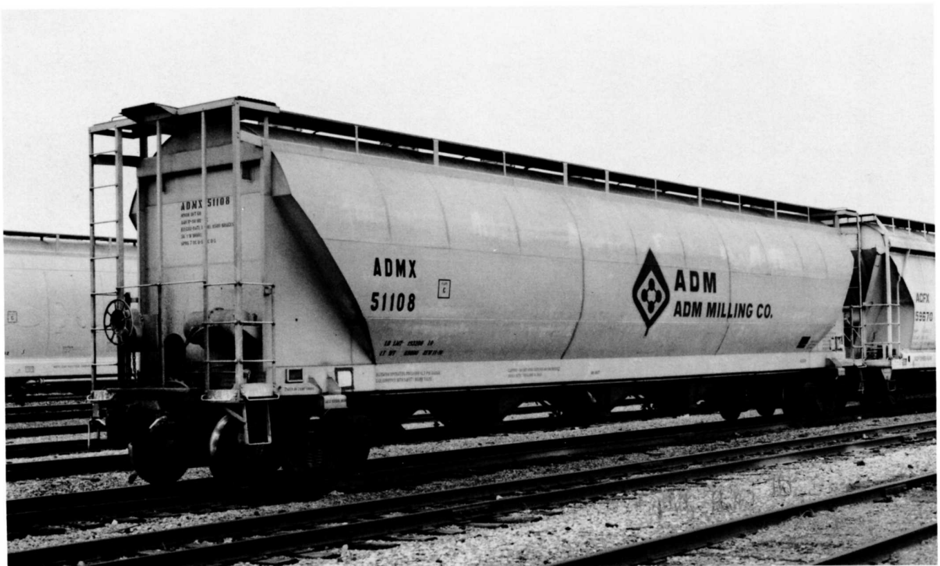
(Below) ADMX 51108 was built in November 1991 by TRN FW. This one has the gray carbody variation. Photographed August 1993 in Kansas City, MO.
