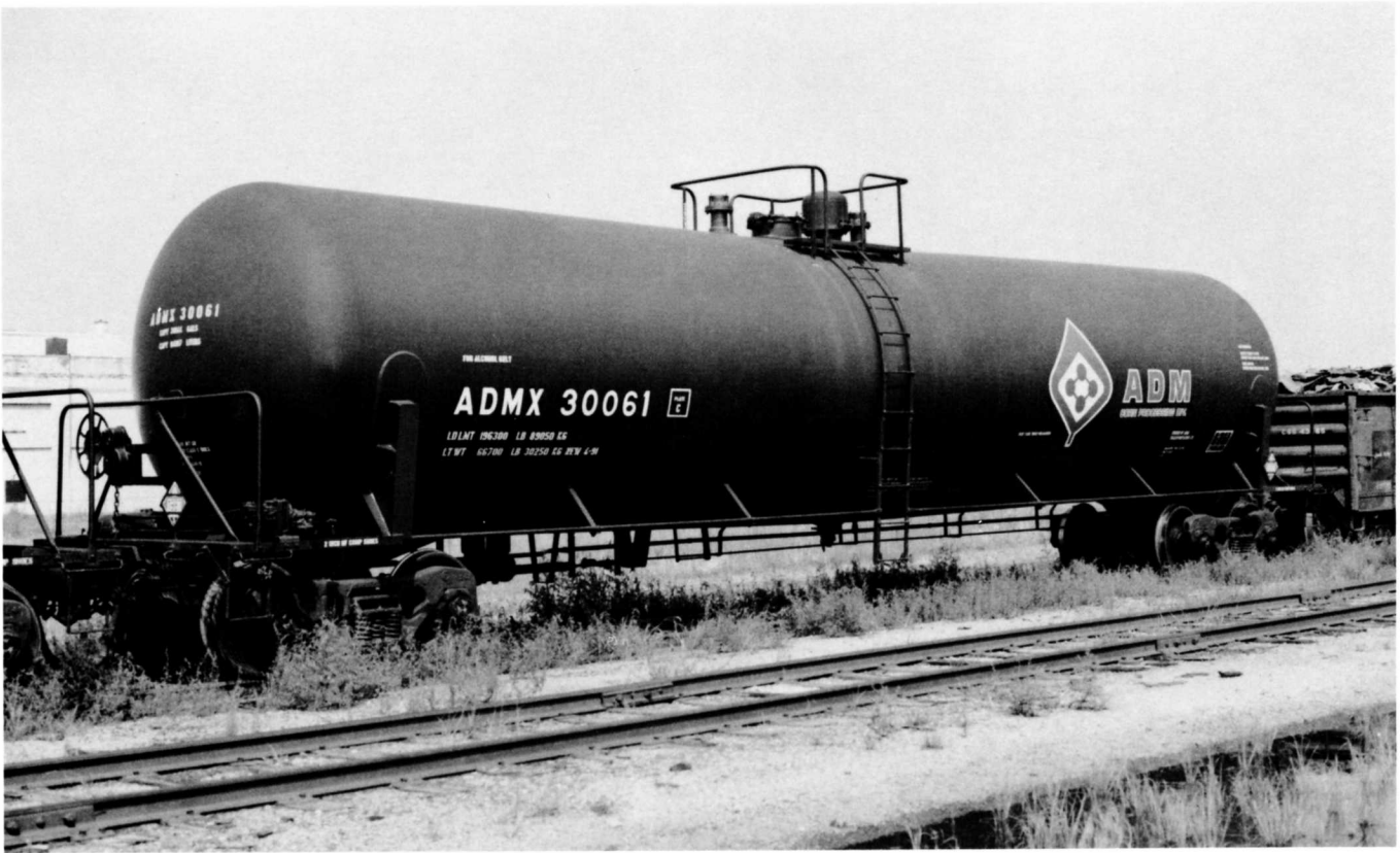
(Above) ADMX 30061 was built in April 1991 by Trinity Oklahoma City (TRN OKC). Note the heavy-duty tank saddles (height on sides of tank). This car is restricted to transporting alcohol. Photographed in Omaha NE in August 1993.
